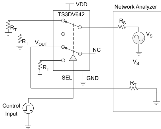
Figure 17. Crosstalk (Xtalk)
