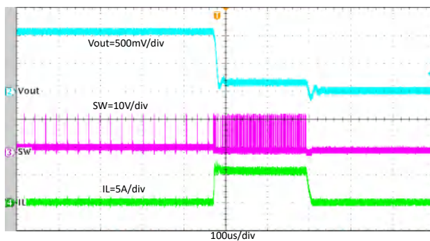
Figure 8-24. TPS564255 Normal Operation to Output Hard Short
