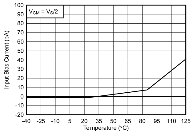
Figure 5-6. Bias Current vs. Temperature, 40V
