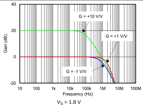
Figure 12. Closed-Loop Gain vs Frequency (Minimum Supply)
