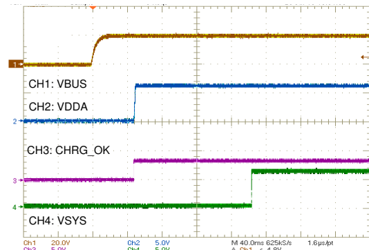
Figure 10-4. Power Up From 20 V
