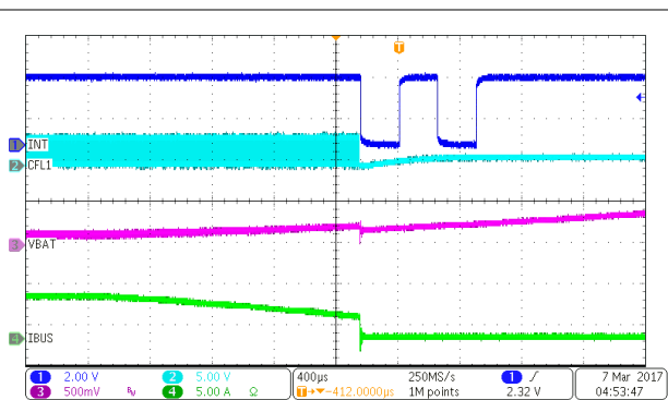
Figure 10-7. VBAT_OVP
