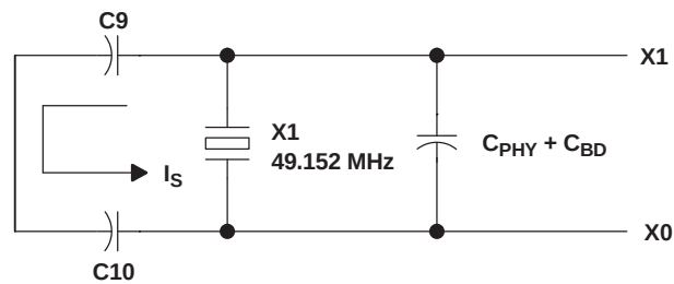
Figure 10. Load Capacitance for the TSB41BA3D PHY
