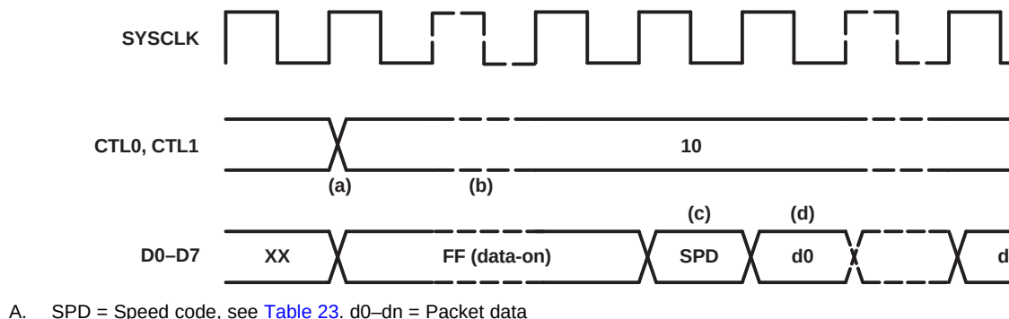
Figure 15. Normal Packet Reception Timing
