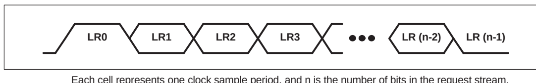
Figure 23. LREQ Request Stream
