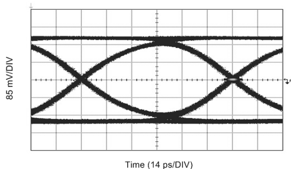
Figure 4. 11.88 Gbps, Input: 20 in. FR4 Trace
