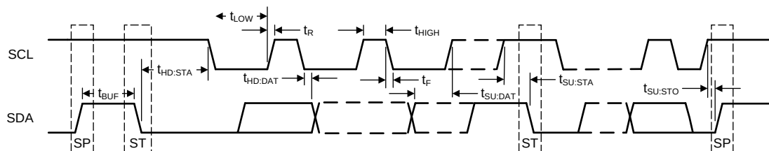
Figure 1. SMBUS Timing Parameters
