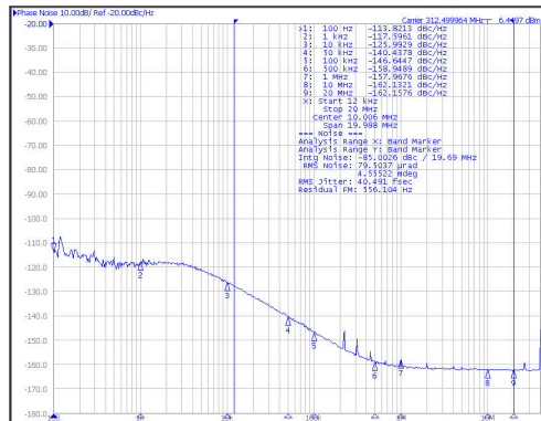
Figure 6-8. 312.5MHz HSDDS Output From BAW APLL
