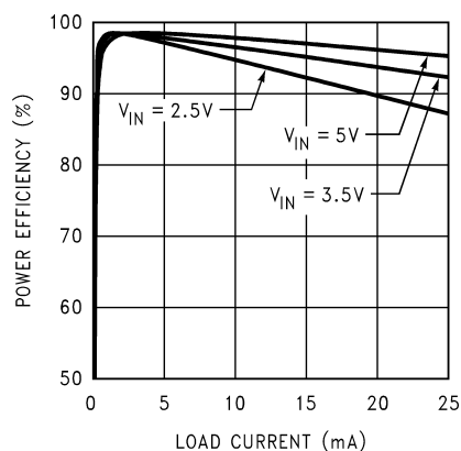
Figure 9-6. Efficiency vs Load Current
