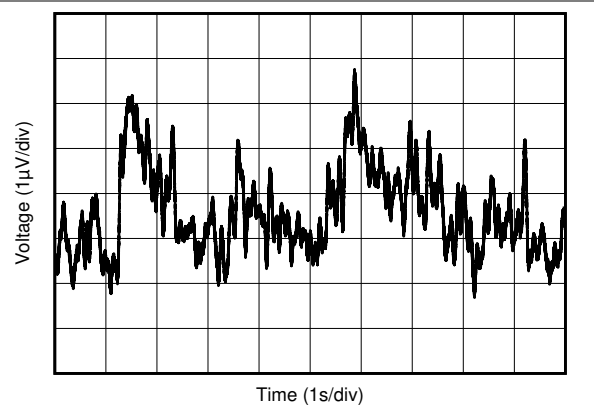
Figure 6-8. 0.1-Hz to 10-Hz Input Voltage Noise
