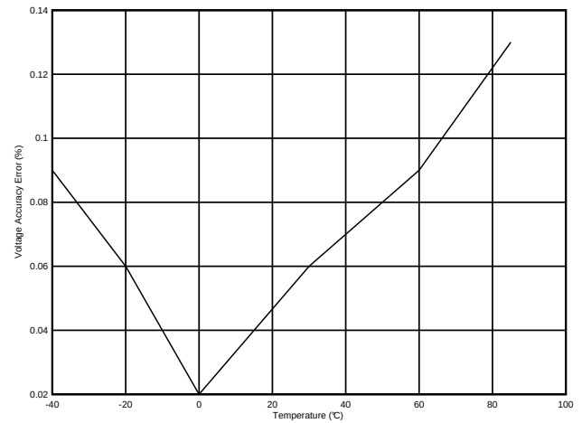
Figure 3. Temperature Accuracy
