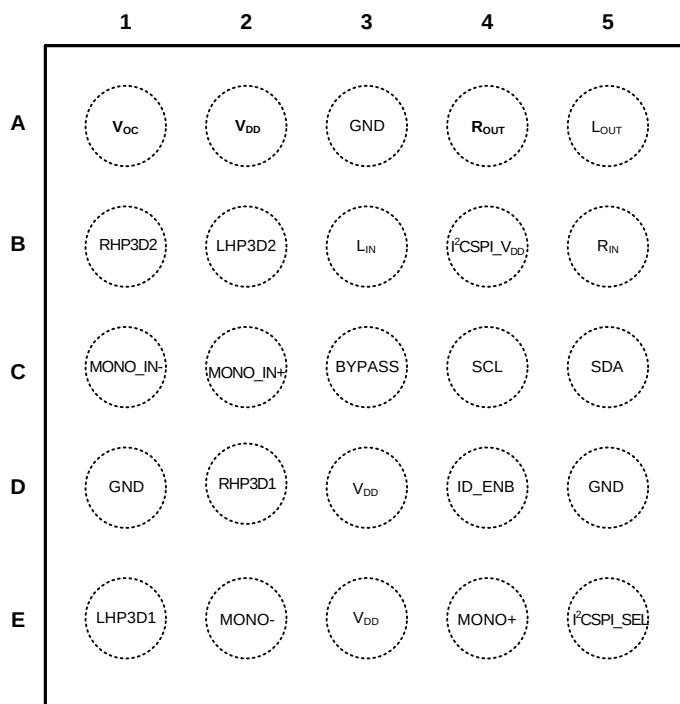
Figure 4. 25 Bump DSBGA Package (Top View)
