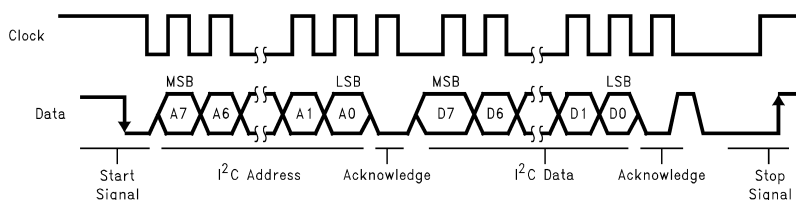
Figure 63. I 2 C Bus Format
