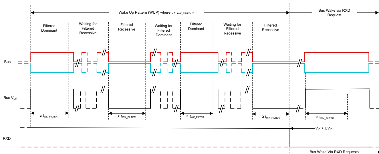
Figure 7-7. Wake-Up Pattern (WUP) with t_{WK\_TIMEOUT}
