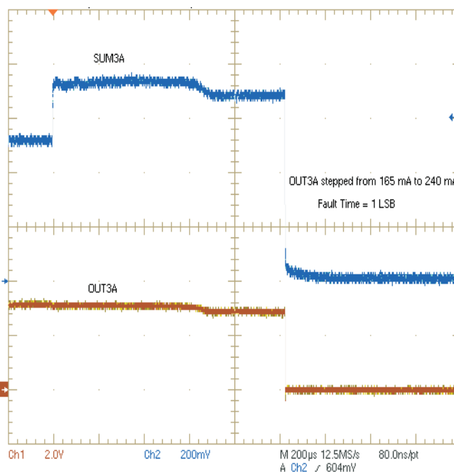
Figure 11. OUT3 Load Stepped from 165 mA to 240 mA
