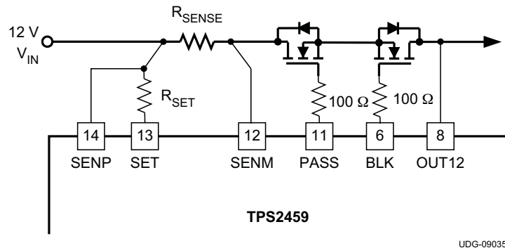
Figure 24. 12-V Path
