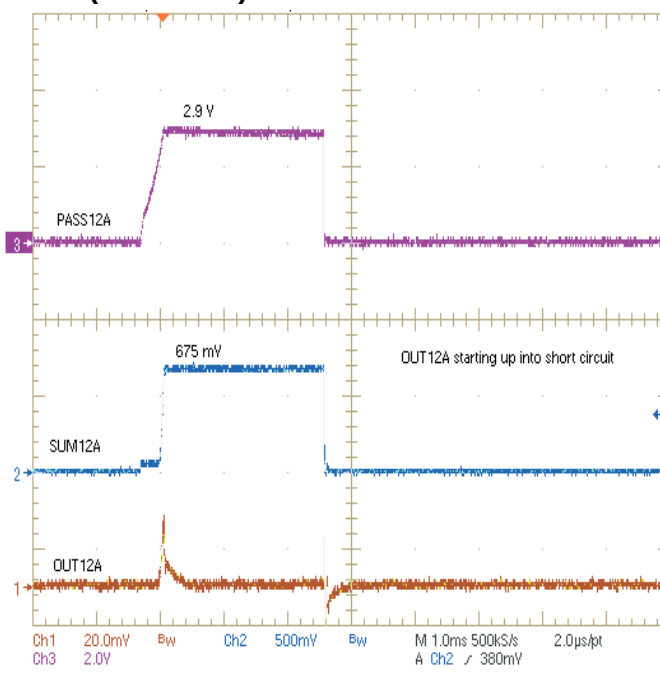
Figure 19. OUT12 Startup Into Short Circuit
