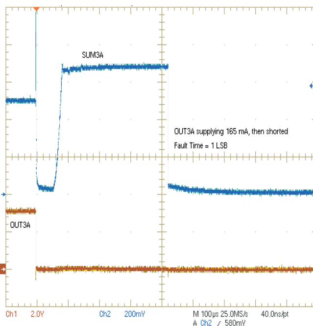
Figure 13. OUT3 Short Circuit Under Full Load, (165 mA), Wide View
