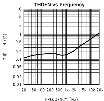
Figure 9. V_{DD} = 12V , R_L = 8\Omega BTL operation, BTLA_V = 20 , P_{OUT} = 3W
