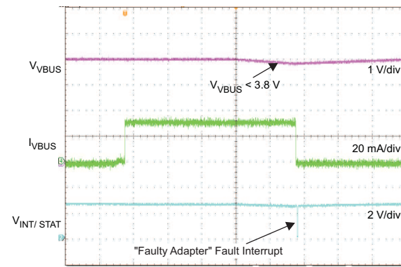
t -Time - 4 ms/div Figure 7. Faulty Adapter Detection
