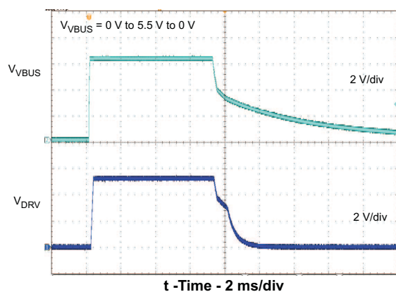
Figure 22. DRV Startup/Shutdown
