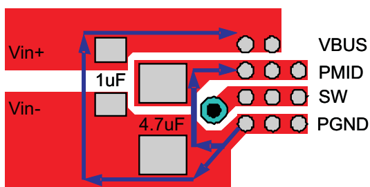
Figure 42. Input Capacitor Position and PCB Layout Example
