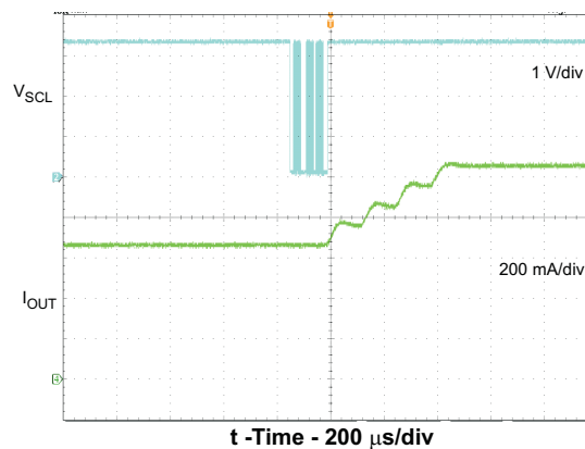
Figure 13. Charge Current Transition 550mA to 1.05A Using I 2 C
