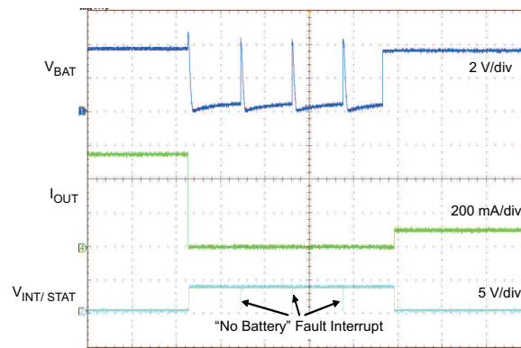
t -Time - 2 s/div Figure 5. Battery Insertion/Removal
