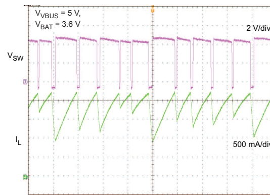
t -Time - 2 μs/div Figure 9. Cycle by Cycle Current Limit
