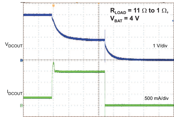
Figure 17. DCOUT OCP Response
