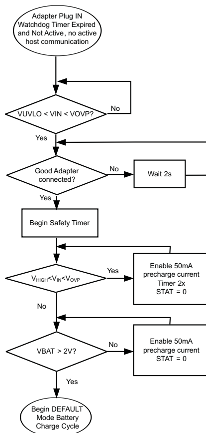
Figure 26. Startup on Adapter Plug-In in DEFAULT Mode
