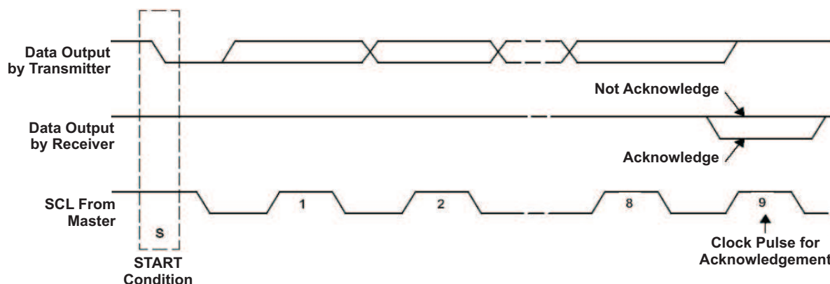
Figure 36. Acknowledge on the I2C Bus
