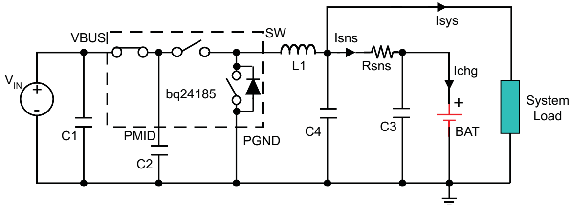
Figure 39. System Load Before Sensing Resistor
