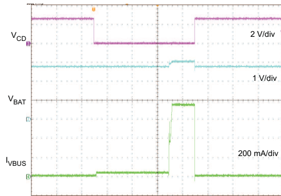
Figure 16. Enable/Disable Using CD
