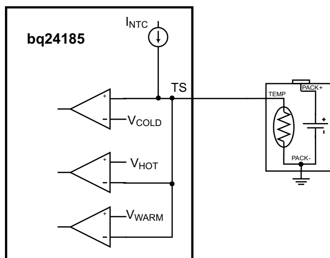
Figure 33. TS Circuit
