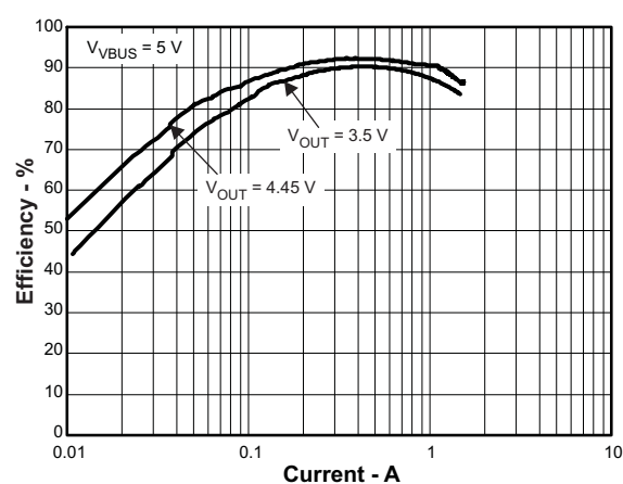
Figure 25. Charger Efficiency
