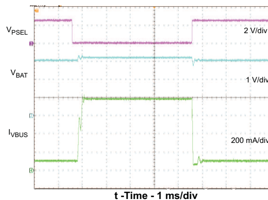
Figure 15. PSEL Transition
