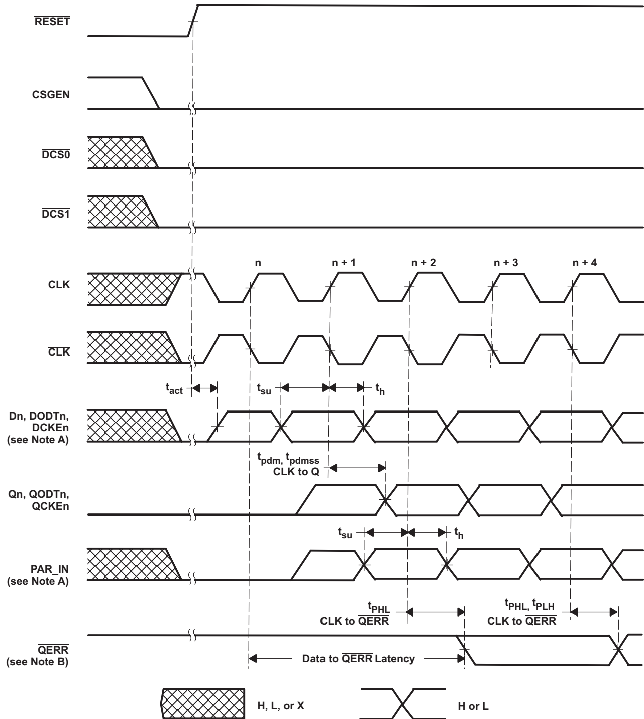
Timing Diagram for 74SSTUB32868A During Start-Up ( \overline{\text{RESET}} Switches From L to H)
