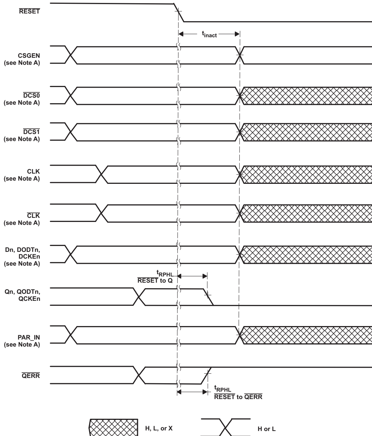
Timing Diagram for 74SSTUB32868A During Shut-Down ( \overline{\text{RESET}} Switches From H to L)
