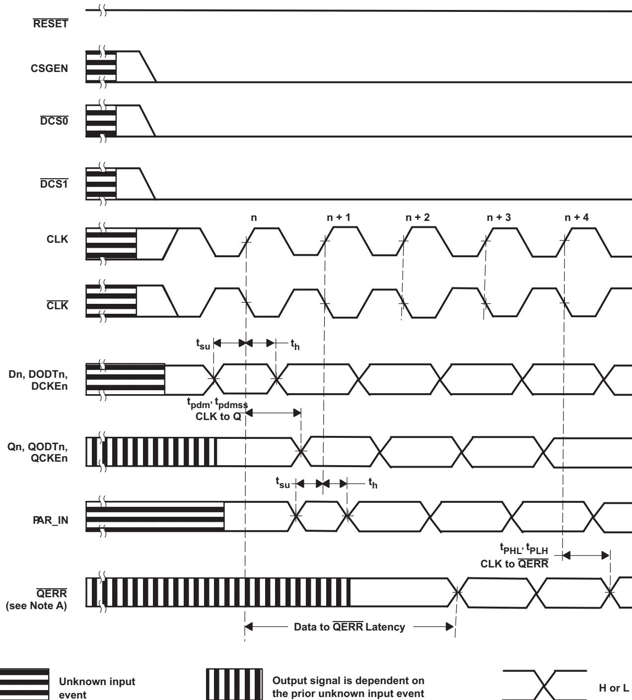
Timing Diagram for 74SSTUB32868A During Normal Operation ( \overline{\text{RESET}} = \text{H} )
