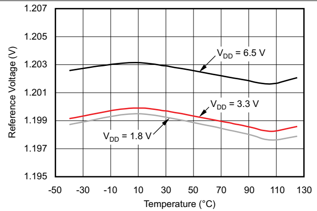
Figure 27. TPS386040 V_{REF} at 0\text{ }\mu\text{A} vs Temperature
