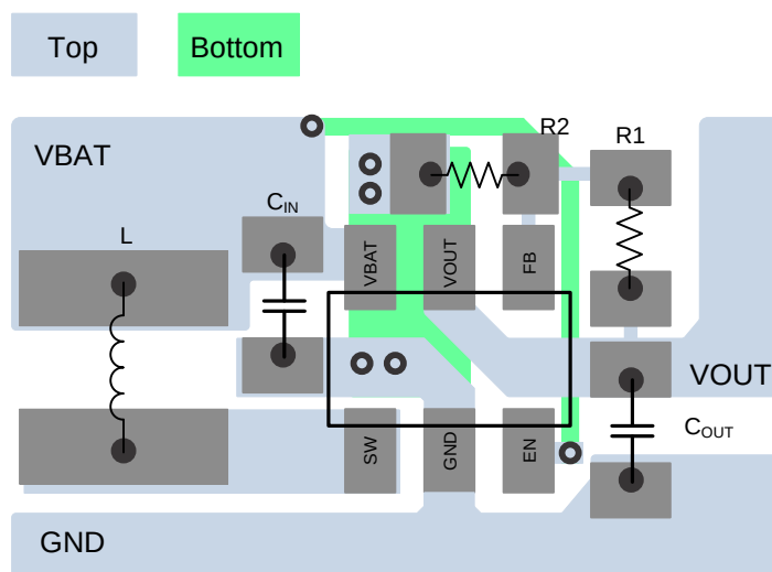
Figure 18. PCB Layout Recommendation
