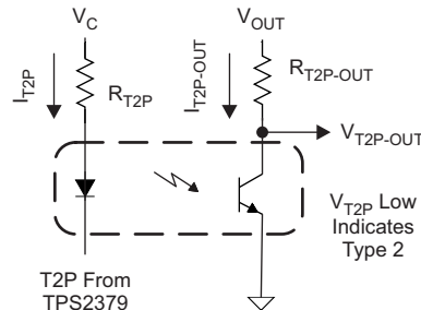
Figure 18. T2P Interface
