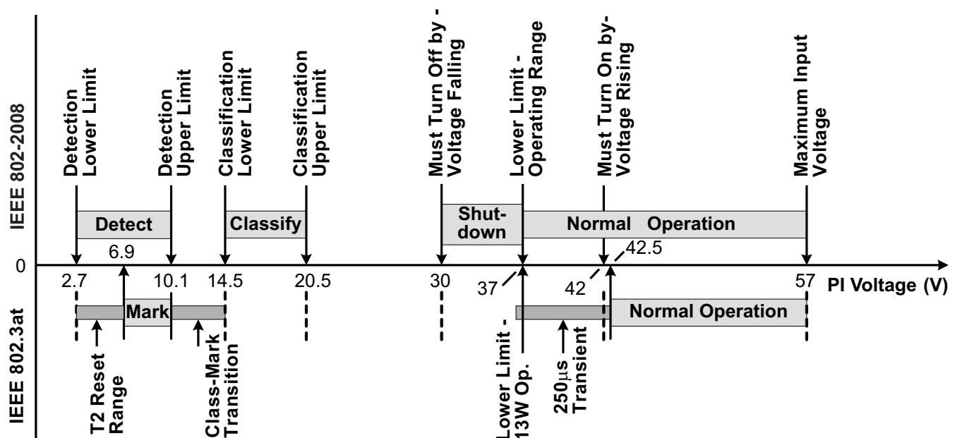
Figure 19. Threshold Voltages
