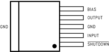
Figure 2. DDPAK/TO-263, Top View
