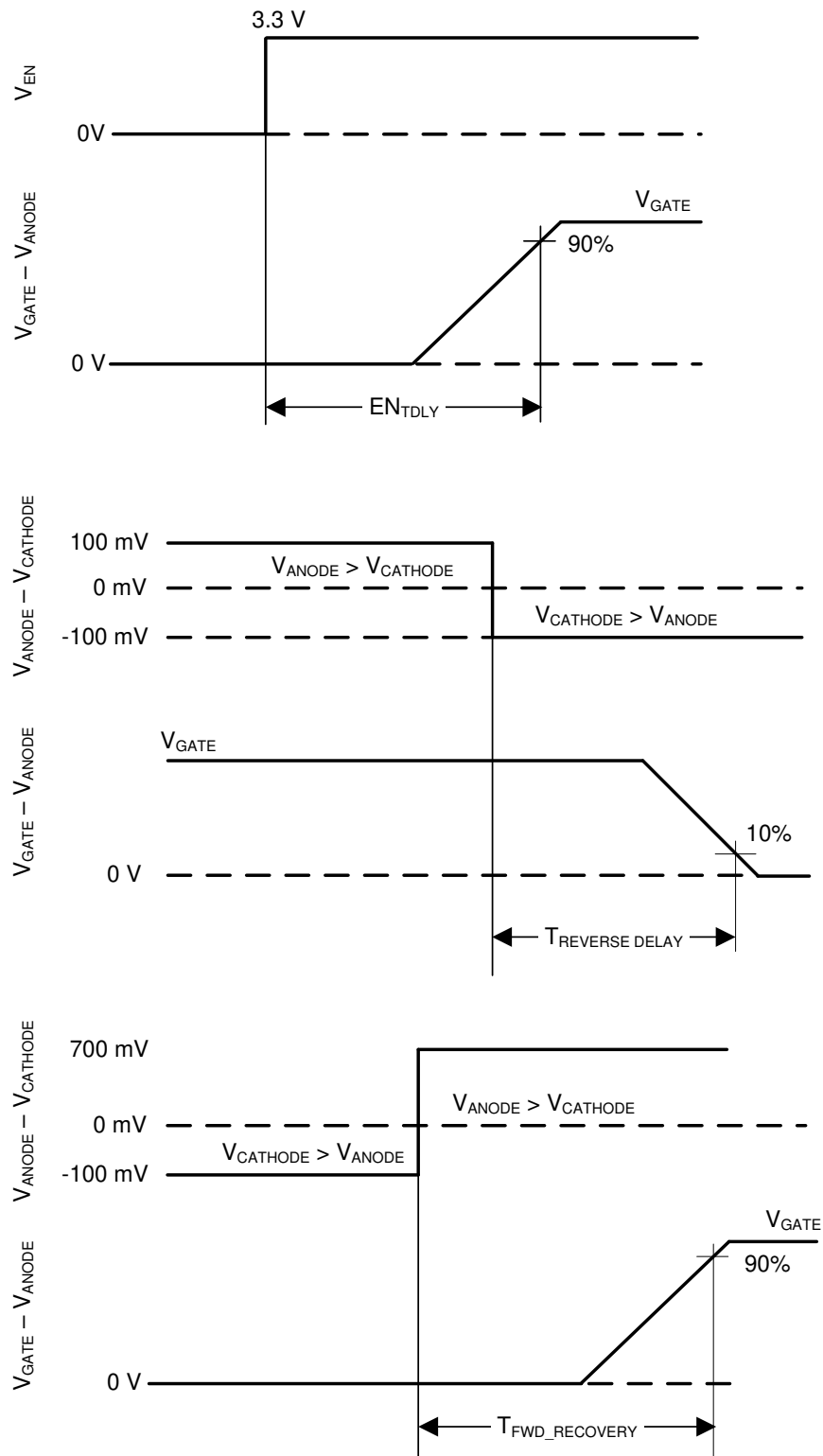
Figure 7-1. Timing Waveforms
