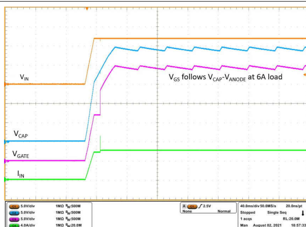
Figure 9-7. Startup With 6-A Load
