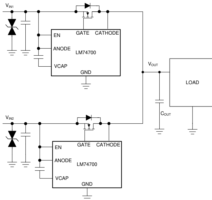
Figure 9-18. Typical OR-ing Application
