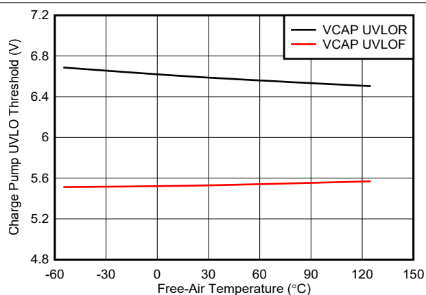
Figure 6-14. Charge Pump UVLO Threshold vs Temperature
