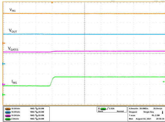
Figure 9-16. ORing – V_{IN2} Failure and Switch Over to V_{IN1}
