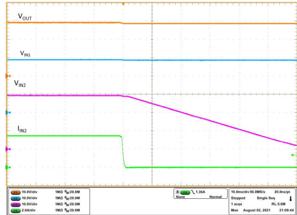
Figure 9-17. ORing - V_{IN2} Failure and Switch Over to V_{IN1}
