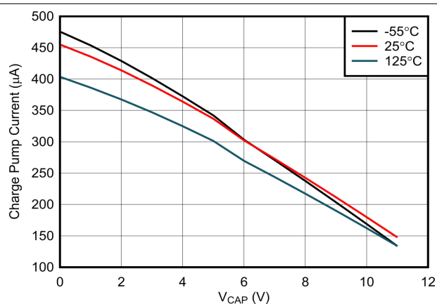
Figure 6-6. Charge Pump V-I Characteristics at V_ANODE >= 12 V
