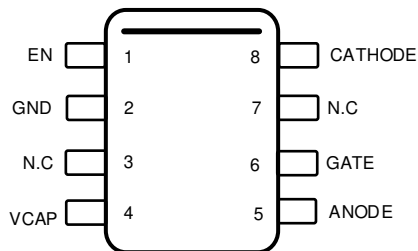
Figure 5-1. DDF Package 8-Pin SOT-23 Top View
