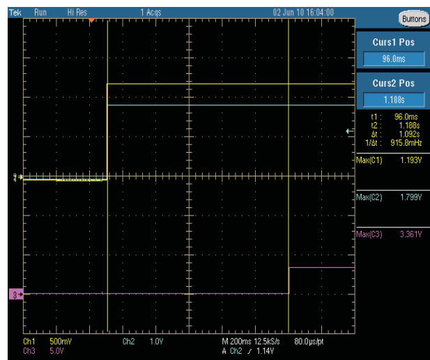
Figure 8. Power Up and PGOOD (From Top to Bottom, Buck2 = 1.8 V, Buck1 = 1.2 V, PGOOD) V_{IN} = 12\text{ V} , f_{SW} = 500\text{ kHz} , L_O = 4.7\text{ }\mu\text{H} , DCR = 10\text{ m}\Omega , C_O = 22\text{ }\mu\text{F}
