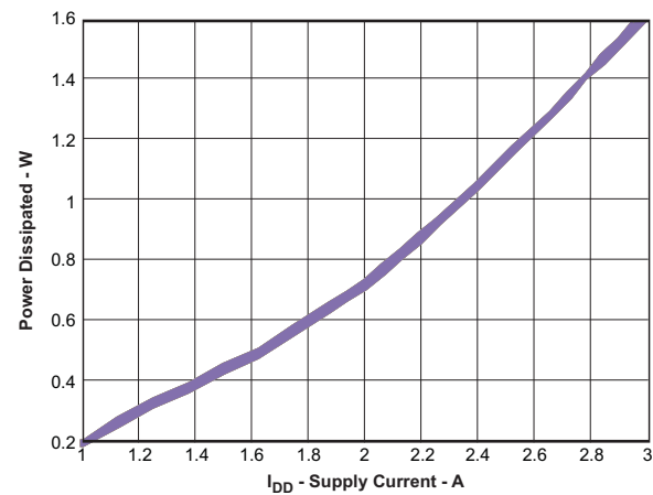
Figure 25. Buck 1 V_{IN} = 5 V, f_S = 500 kHz, V_O (From Top to Bottom) = 5, 3.3, 2.5, 1.8, 1.2 V
