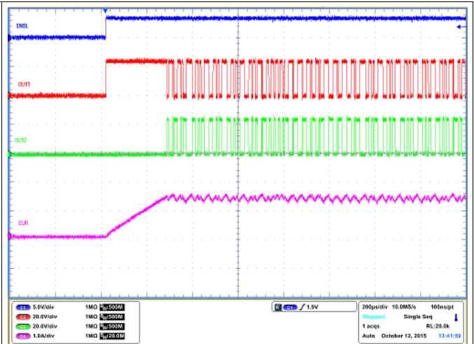
Figure 9. DRV8842 Direction Change
