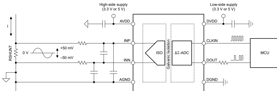
Typical Application
