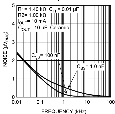
Figure 21. Output Noise
