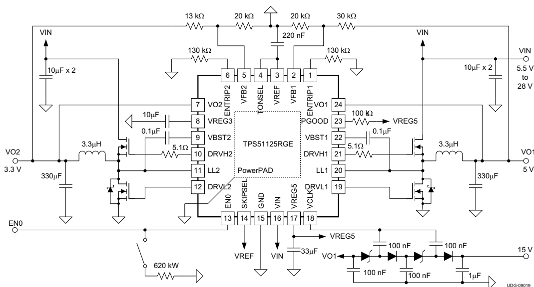
Simplified Schematic
