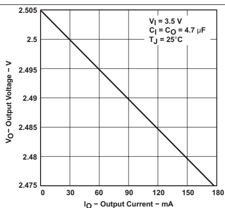
Figure 1. TPS76325-Q1 Output Voltage vs Output Current
