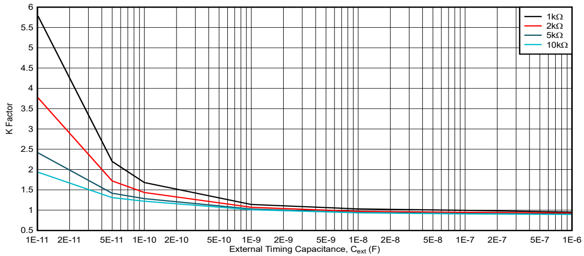
Figure 5-10. K Factor, V_{CC} = 3.3V , R_{ext} = 1k\Omega to 10k\Omega
