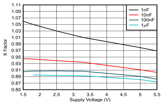
Figure 5-3. K Factor vs Supply Voltage, R_{\text{ext}} = 10\text{k}\Omega
