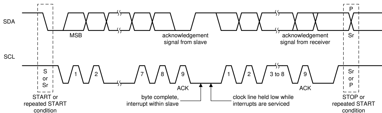
Figure 7-7. Bus Protocol
