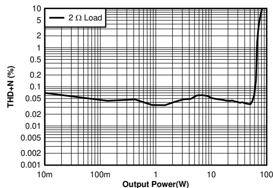
Figure 6-19. THD+N vs Power - PBTL, 2 \Omega , 18 V
