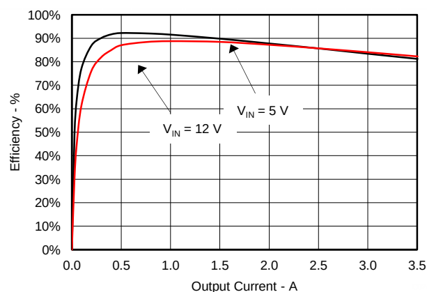
Figure 3. 1.8-V Efficiency
