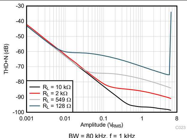
Figure 6-24. THD+N vs Output Amplitude
