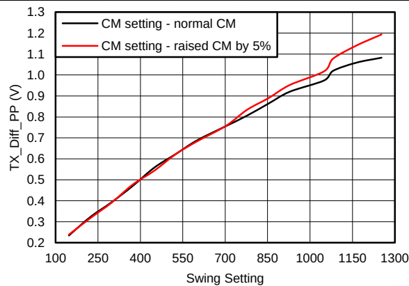
Figure 4-7. TX Termination I-V
