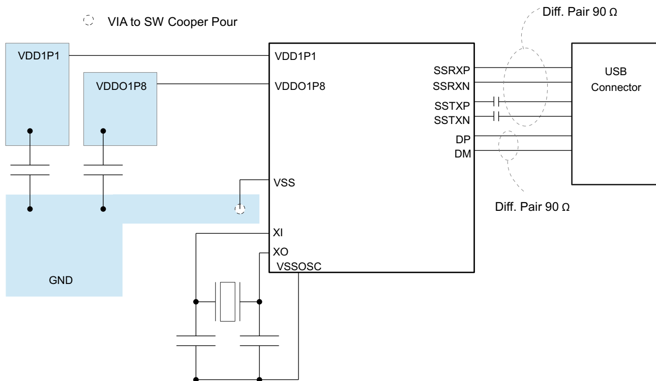
Figure 6-7. Layout Example
