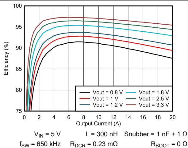
Figure 5-2. TPS546B24S Efficiency vs Output Current
