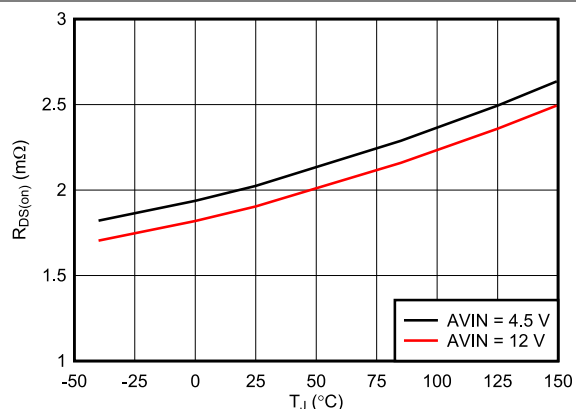
Figure 5-6. Low-Side MOSFET On-Resistance ( R_{DS(on)} ) vs Junction Temperature
