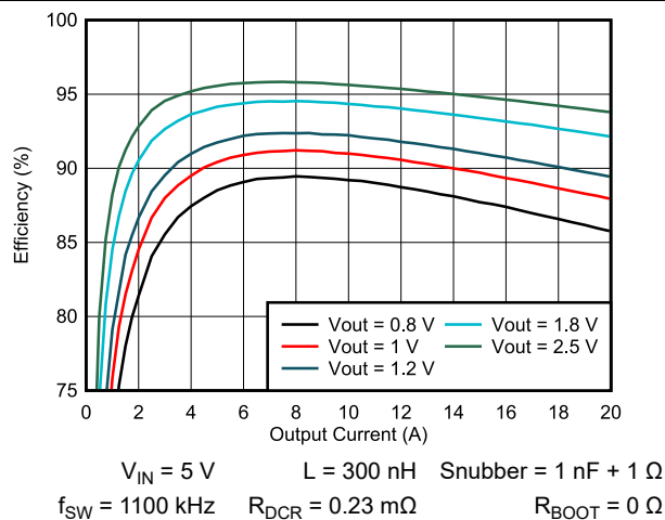
Figure 5-3. TPS546B24S Efficiency vs Output Current
