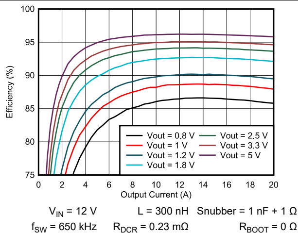
Figure 5-4. TPS546B24S Efficiency vs Output Current
