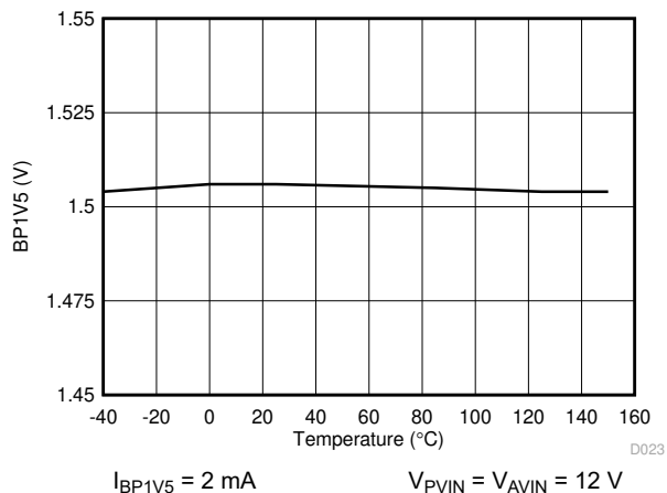
Figure 5-12. BP1V5 Voltage vs Junction Temperature
