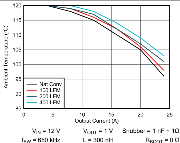
Figure 5-1. TPS546B24S Safe Operating Area
