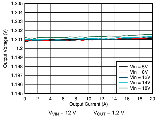
Figure 7-3. Load Regulation
