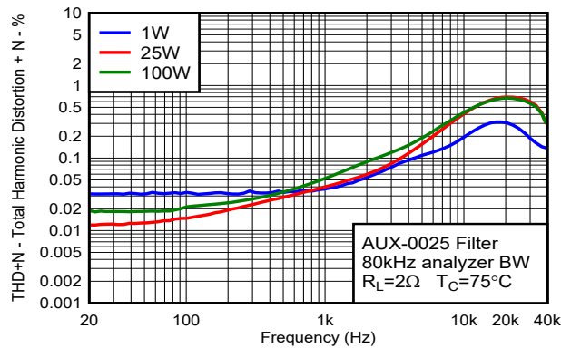
Figure 7-19. Total Harmonic Distortion+Noise vs Frequency
