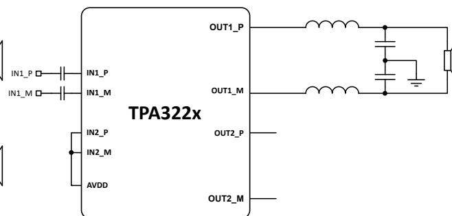
Figure 9-11. Mono BTL
