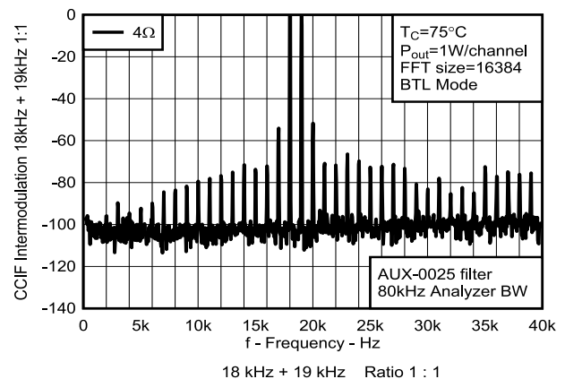
Figure 7-12. CCIF Intermodulation
