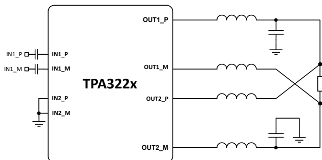
Figure 9-12. Mono PBTL, Post LC Filter
