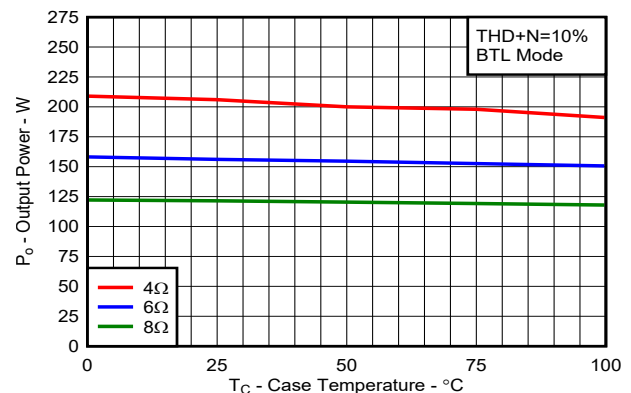
Figure 7-10. Output Power vs Case Temperature
