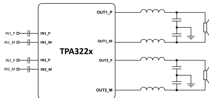
Figure 9-10. Stereo BTL
