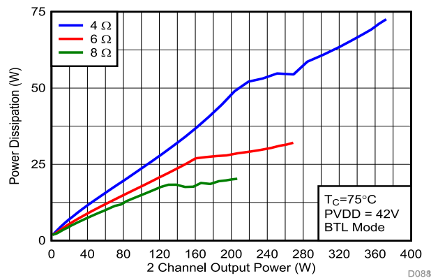
Figure 7-9. Power Dissipation vs Output Power
