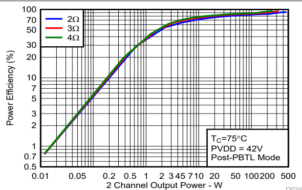
Figure 7-21. System Efficiency vs Output Power
