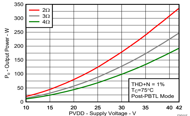
Figure 7-20. Output Power vs Supply Voltage
