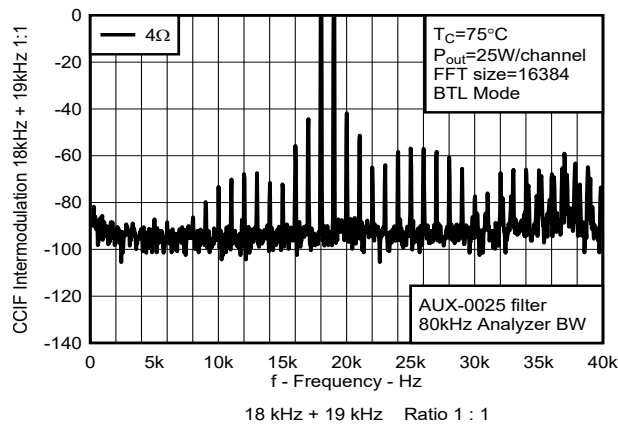
Figure 7-13. CCIF Intermodulation
