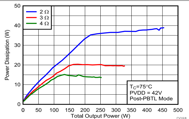
Figure 7-22. Power Dissipation vs Output Power
