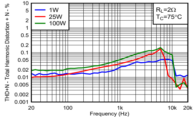
Figure 7-18. Total Harmonic Distortion+Noise vs Frequency
