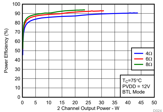
Figure 7-8. System Efficiency vs Output Power
