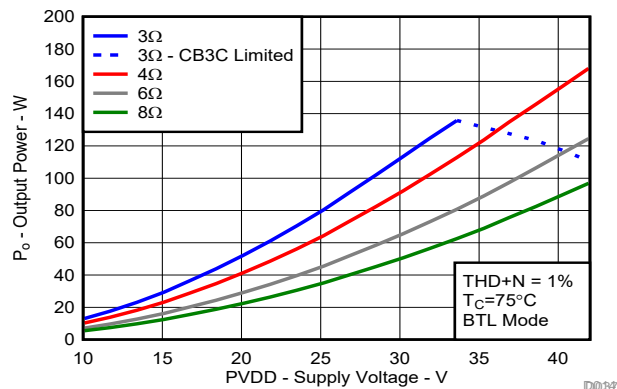
Figure 7-5. Output Power vs Supply Voltage, AD-mode
