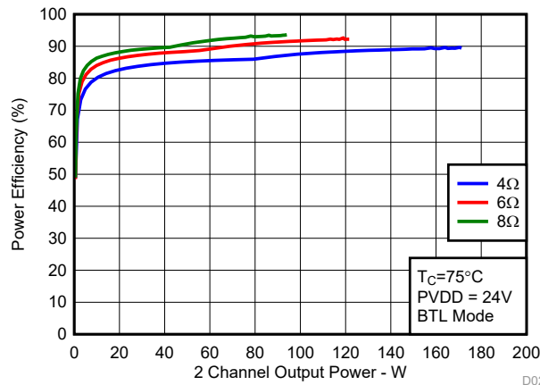
Figure 7-7. System Efficiency vs Output Power
