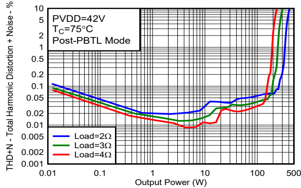
Figure 7-17. Total Harmonic Distortion+Noise vs Output
