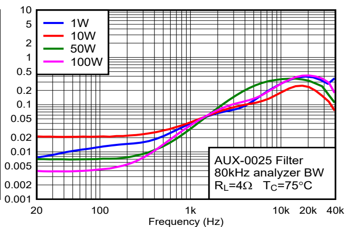
Figure 10-3. Total Harmonic Distortion+Noise vs Frequency
