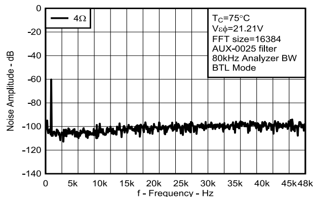
Figure 7-11. Noise Amplitude vs Frequency
