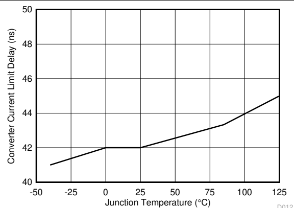
Figure 6-18. Converter Current Limit Delay vs Temperature
