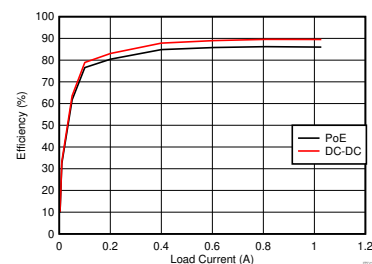
Efficiency Vs. Load Current, 12 V Output
