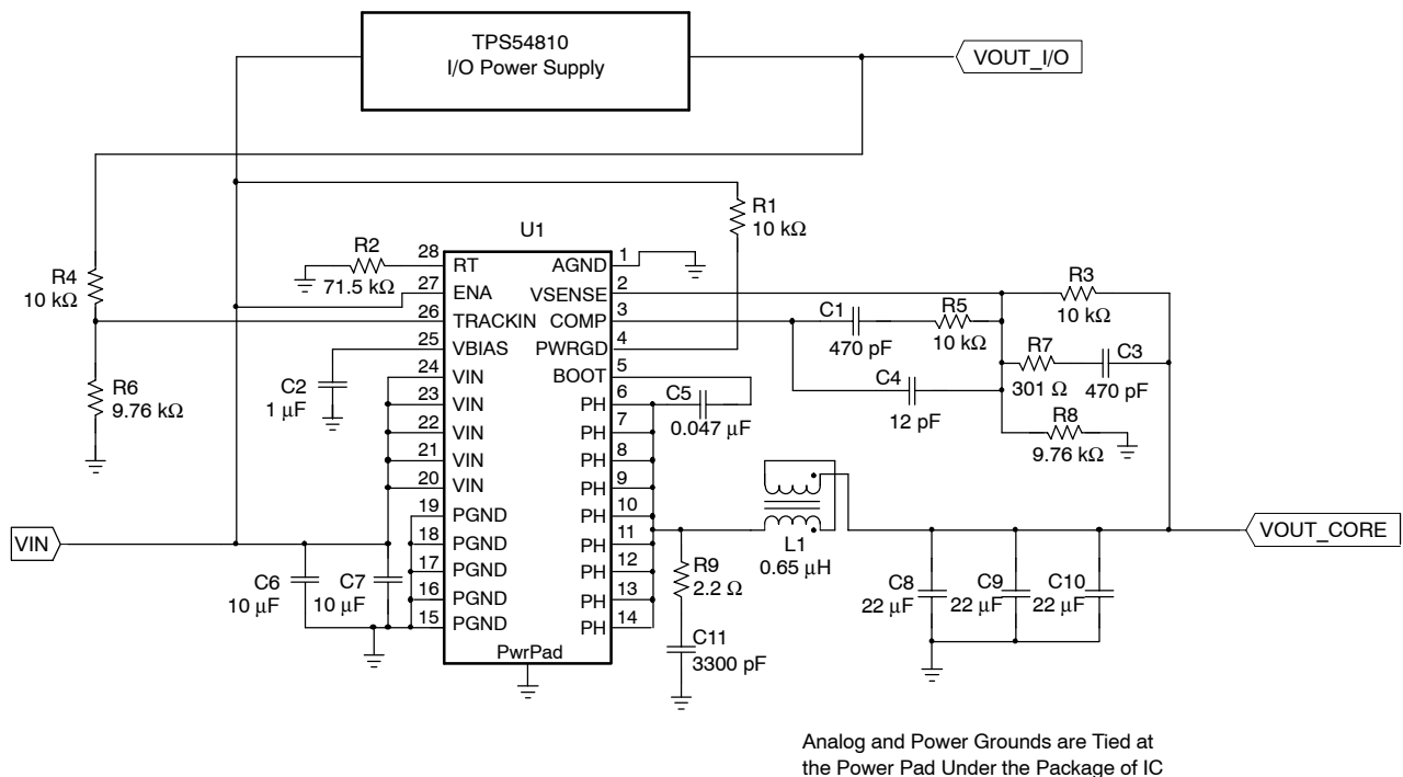
Figure 8. Application Circuit
