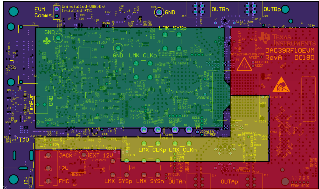
Layer5 / PWR2 DAC VDDL = RED DAC VDDLb = YELLOW DAC VDDCLK1P0V = GREEN Figure 8-31. Power Plane Layout for Layer 5
