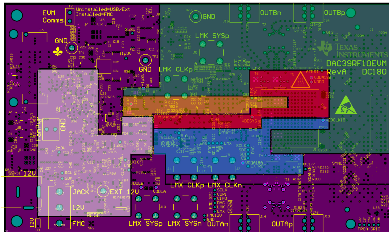
Layer12 / PWR3 DAC VDDA18A = RED DAC VDDA18B = ORANGE DAC VDDDB = YELLOW DAC VEExA = GREEN DAC VEExB = BLUE VDDIO = WHITE Figure 8-32. Power Plane Layout for Layer 12
