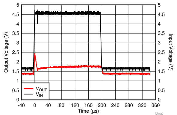
Figure 5-25. V_{IN} Transient From 1.5V to 4.5V
