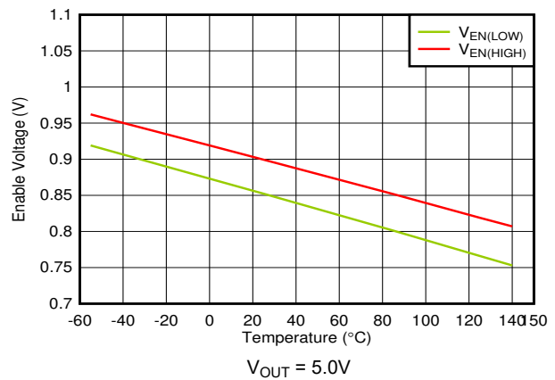
Figure 5-38. EN High and Low Threshold vs Temperature
