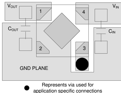
Figure 7-6. Layout Example for DQN Package
