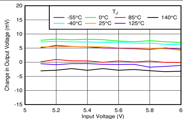
Figure 5-27. Output Accuracy vs V_{IN} and Temperature
