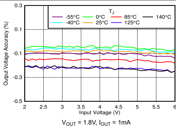
Figure 5-27. Output Accuracy vs V_{IN} and Temperature
