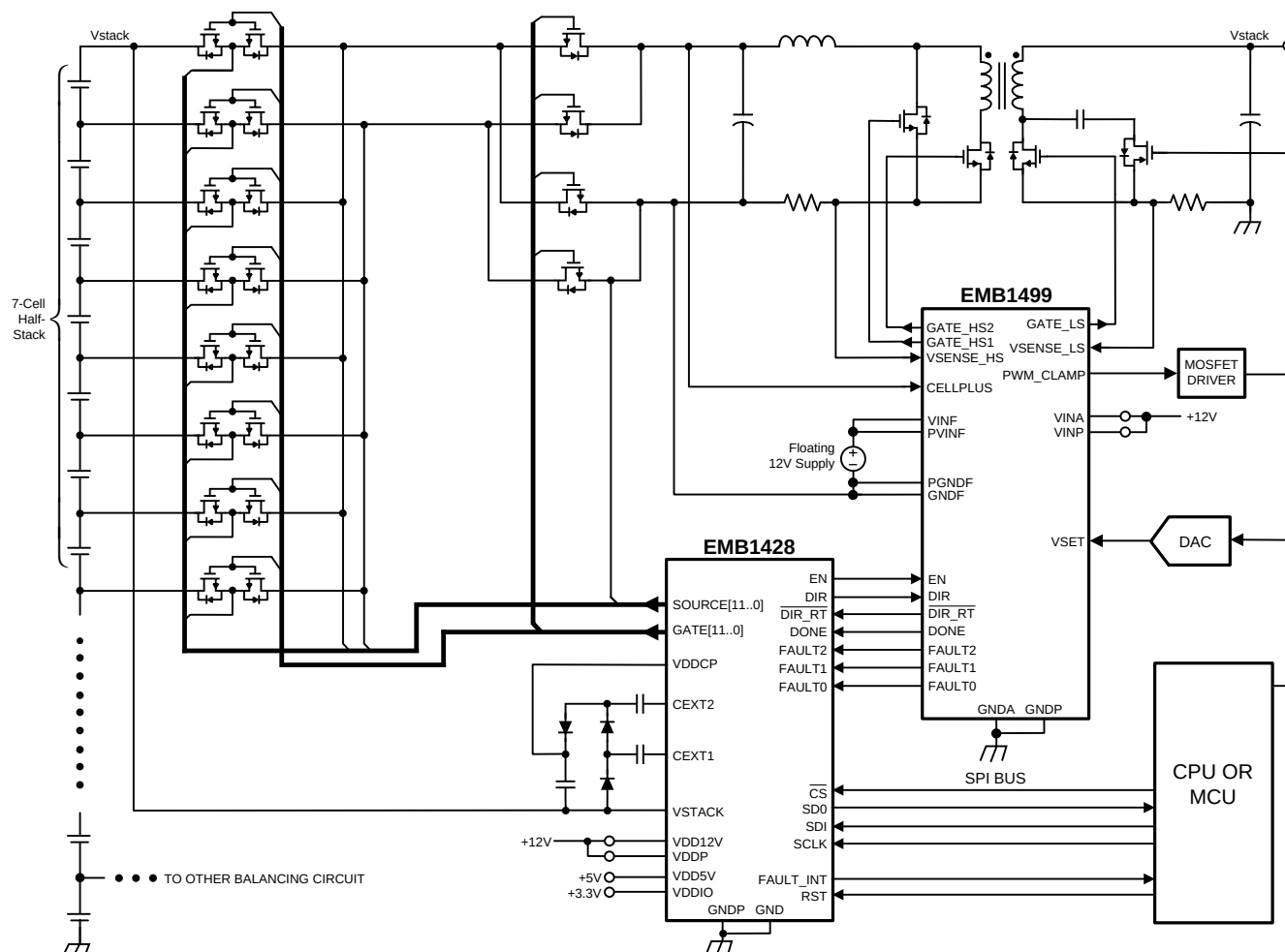
Figure 1. Typical Application
