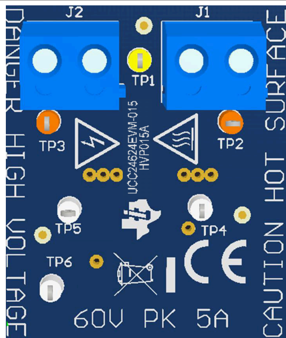
Figure 11-2. UCC24624EVM-015 (Top View)
