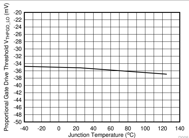
Figure 7-5. Proportional Gate Drive Threshold vs Temperature
