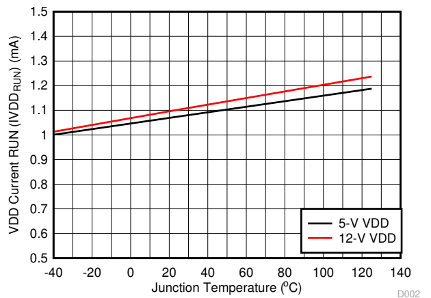
Figure 7-2. Bias Supply Current vs Temperature (No Switching)
