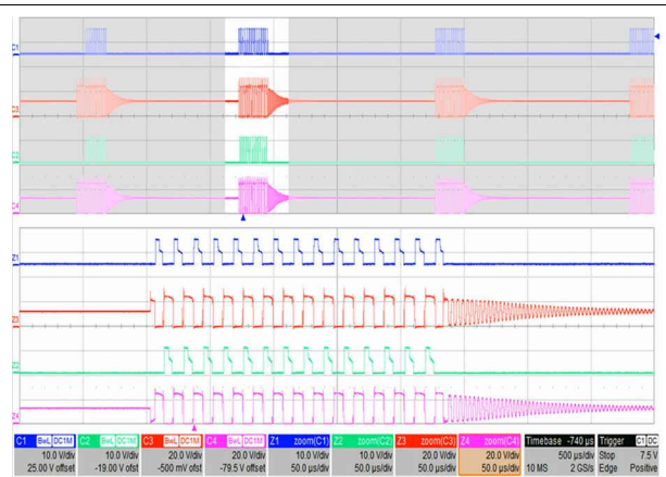
Figure 9-3. V_{IN} = 340 \text{ V} , I_{OUT} = 0.3 \text{ A} , LLC is Operating In Burst Mode
