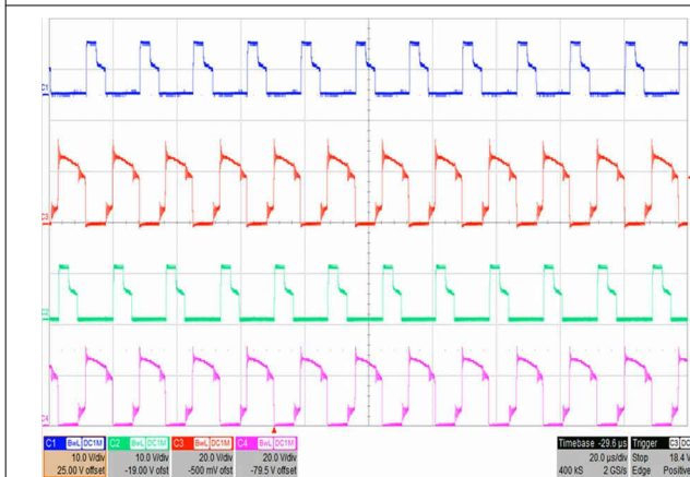
Figure 9-4. V_{IN} = 340 \text{ V} , I_{OUT} = 10 \text{ A} Full Load
