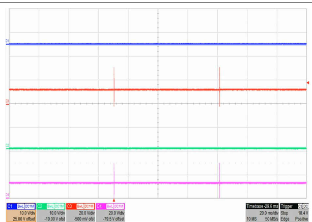
Figure 9-5. V_{IN} = 390 \text{ V} , I_{OUT} = 0 \text{ A} , No Gate Drive Under Light Load (VG1, VG2)
