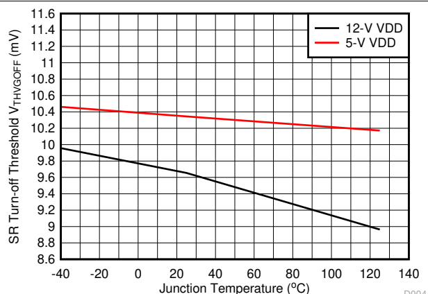
Figure 7-4. SR Turn-off Threshold Voltages vs Temperature
