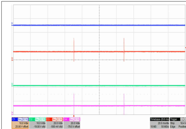
Figure 9-2. V_{IN} = 340 \text{ V} , I_{OUT} = 0 \text{ A} , No Gate Drive Under Light Load (VG1, VG2)
