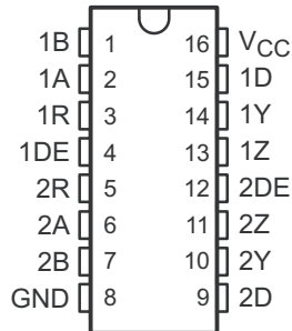
Figure 4-2. SN65C1168: N, NS, or PW Package SN75C1168: DB, N, NS, or PW Package (Top View)
