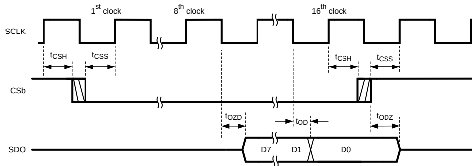
Figure 25. Read Timing
