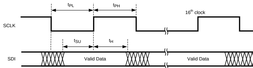
Figure 26. Write Timing
