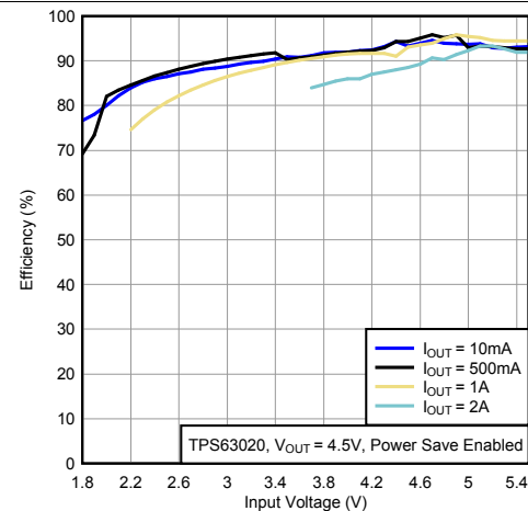
Figure 13. Efficiency Versus Input Voltage, TPS63020, V_{OUT} = 4.5\text{ V} , Power Save Enabled
