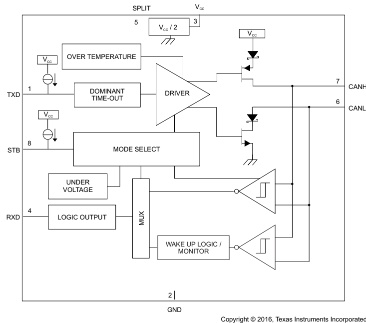
Figure 14. HVDA553 Block Diagram
