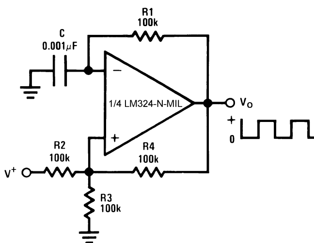
Figure 25. Squarewave Oscillator
