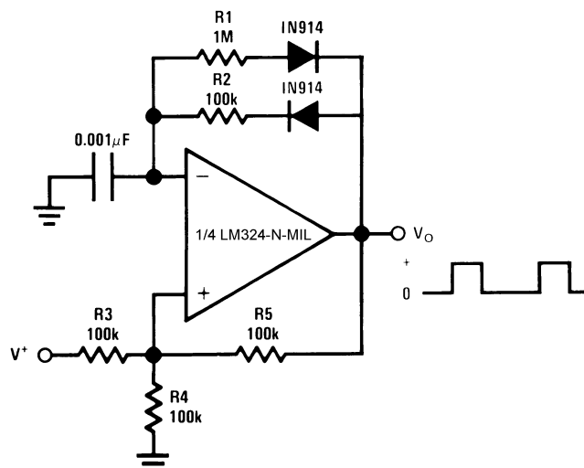
Figure 24. Pulse Generator
