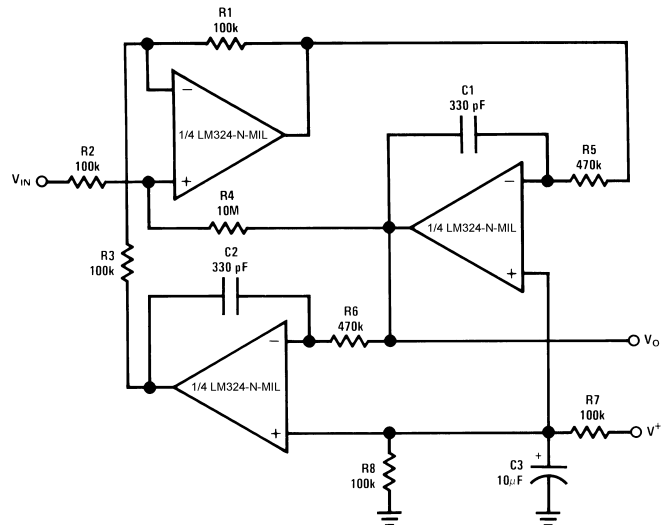
Figure 16. Power Amplifier
