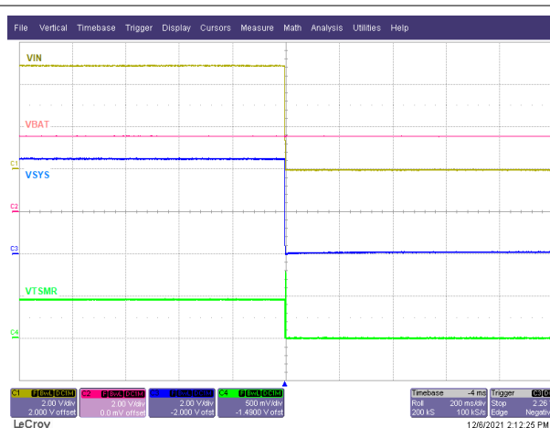
Figure 9-7. Enter Shipmode with Push Button Long Press
