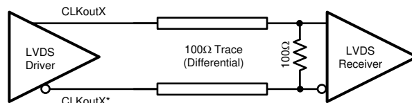
Figure 10-6. Differential LVDS Operation, DC Coupling, No Biasing by the Receiver
